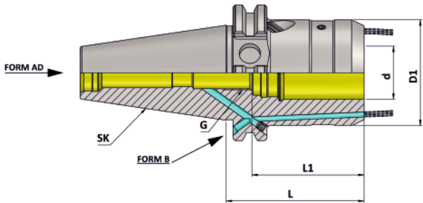
SK (DIN 69871) Hydraulic Expansion Chuck (FCC - AD+B)
