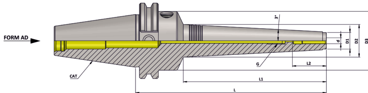
CAT (ANSI B 5.50) Hydraulic Expansion Chuck Slim 3 Degree
