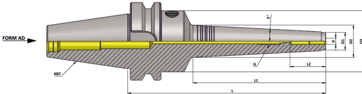
KBT (MAS 403) Hydraulic Expansion Chuck Slim 3 Degree (AD) (JD)
