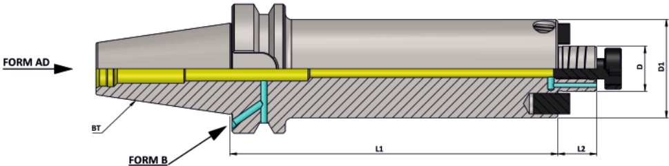
BT (MAS 403) Hydraulic Expansion Face Mill Holder (HC-FMH-K) (Balanced to 2.5 G 25000 RPM)
