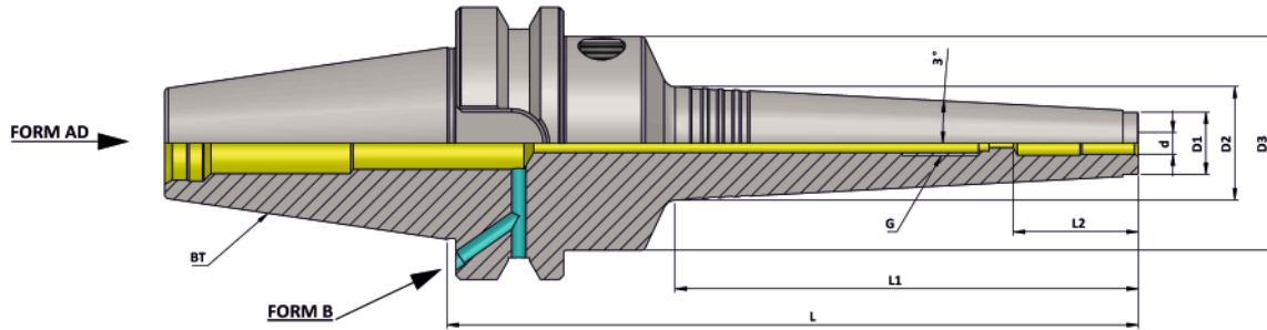
BT (MAS 403) Hydraulic Expansion Chuck Slim 3 Degree (AD+B) (JD/JF)
