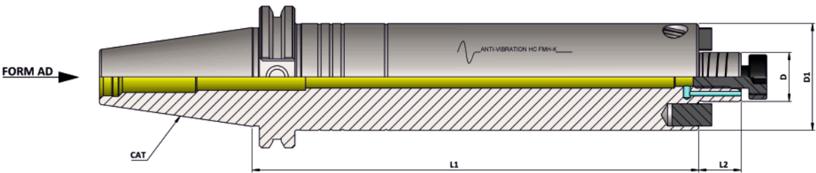
CAT (ANSI-B 5.50) Hydraulic Expansion Face Mill Holder (HC-FMH-K - AD/AV))
