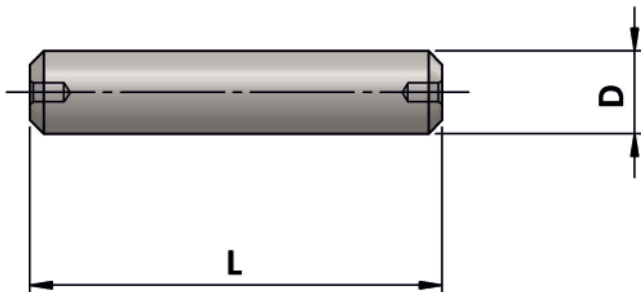
Hydraulic Expansion Chuck Run Out Test Mandrells
