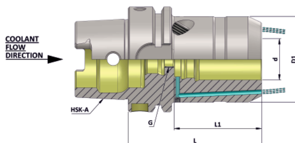
HSK-A (DIN 69893 - 1) Hydraulic Expansion Chuck (FCC)
