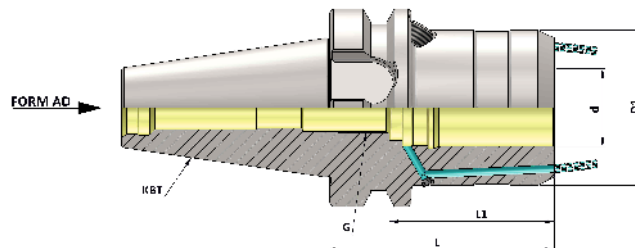
KBT (MAS 403) Hydraulic Expansion Chuck (FCC - AD)
