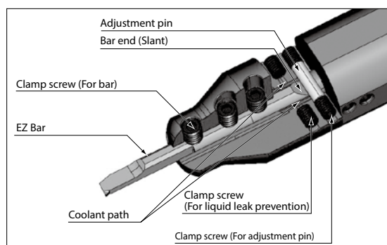
Structure of EZH-CT
