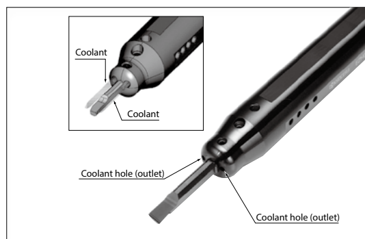
Coolant discharge system of EZH-CT
