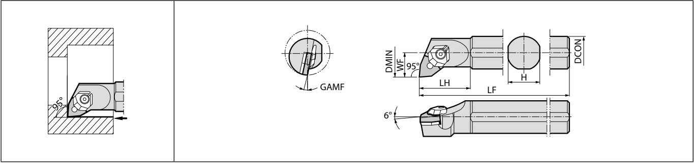
Max. Overhang Length L/D≈5 | Right-hand shown Left-hand Insert for Right-hand Toolholder, Right-hand Insert for Left-hand Toolholder.
