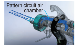
Air cap sectional shape
